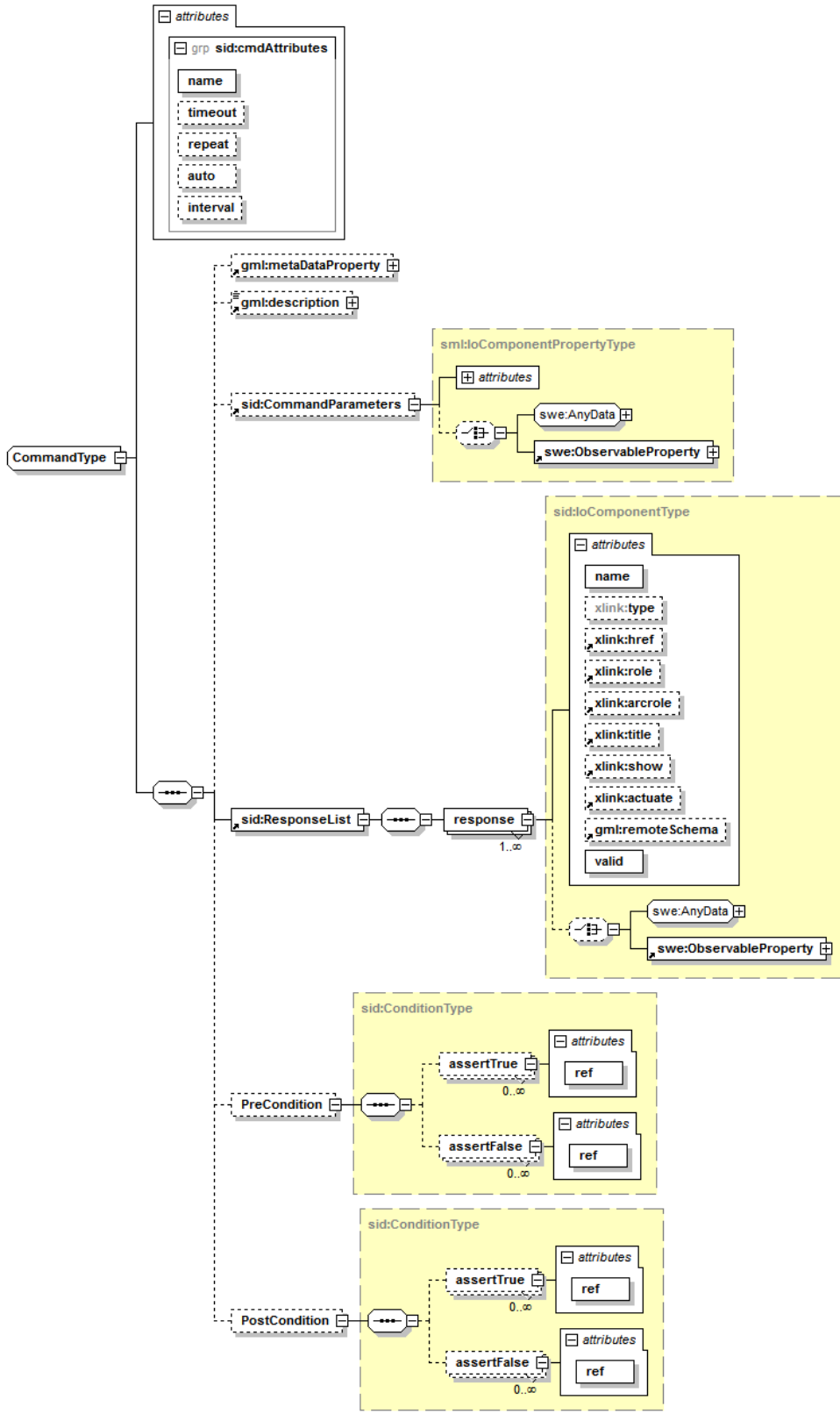
Figure 9 - SID CommandType
