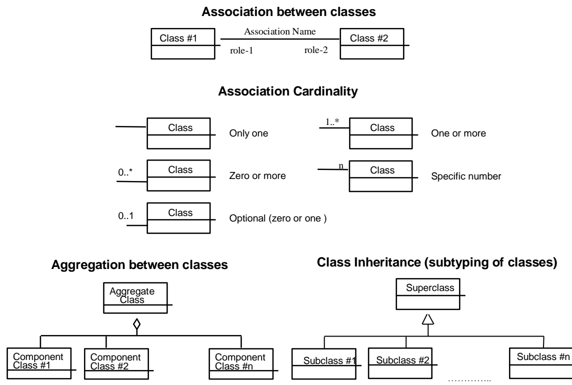
Figure 1 - UML notations
