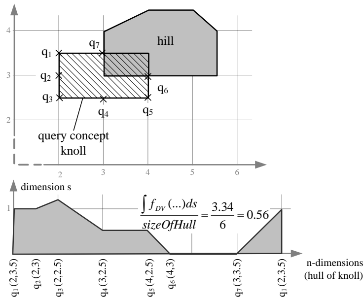
Fig. 11. Overlapping concepts and their semantic distance function.
