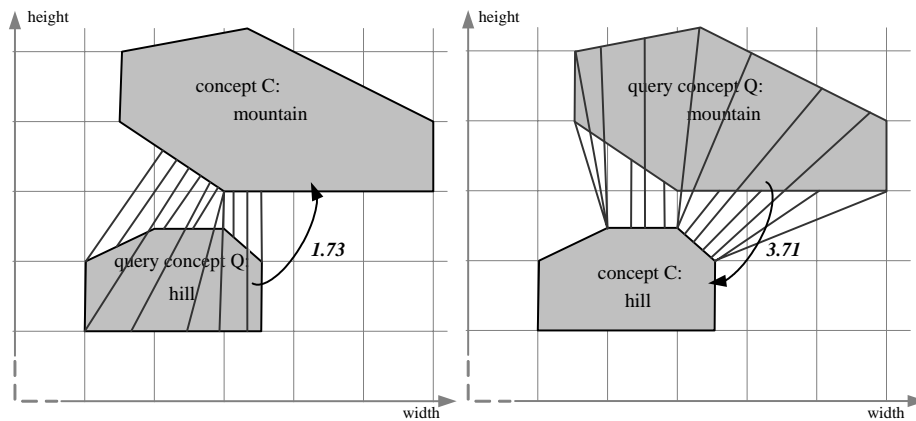
Fig. 9. Asymmetric semantic distance between two concepts.
