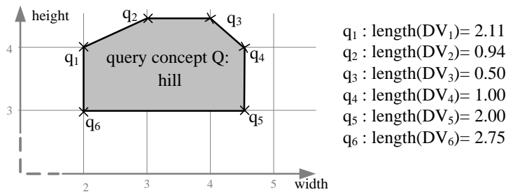
Fig. 5. Distances illustrated as values for each point q_i .
